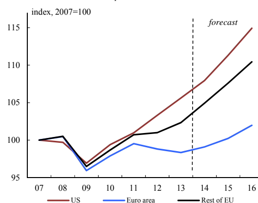
Graph I.5: Real GDP
