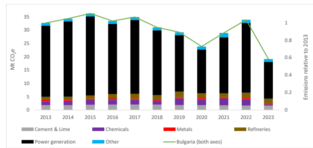
Graph A9.1: ETS emissions by sector since 2013
